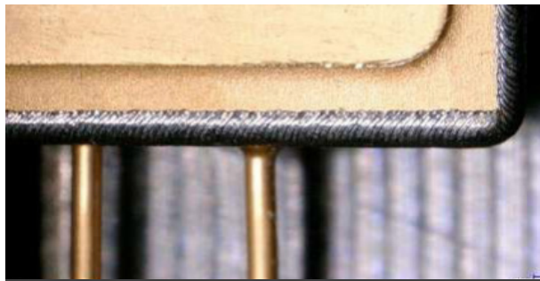
40x magnification of the finished weld.
